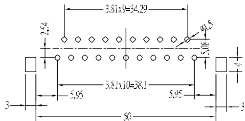
PCB HOLE PATTERN
