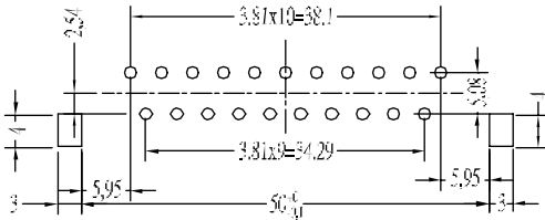
PCB HOLE PATTERN
