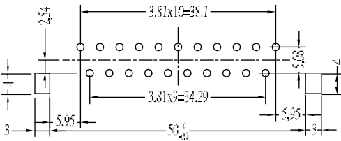
PCB HOLE PATTERN
