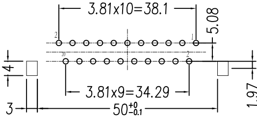
PCB HOLE PATTERN
