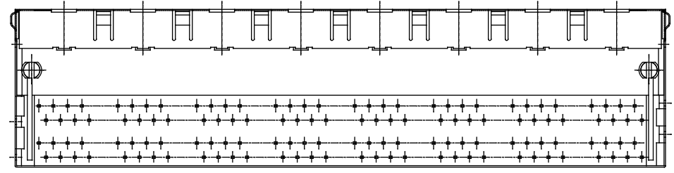
PCB LAYOUT/TOP VIEW
