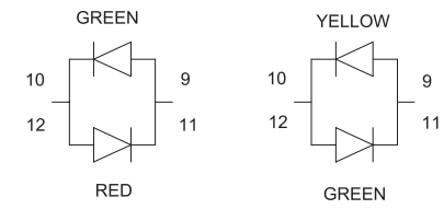
BI-COLOUR LED DETAIL (GREEN/RED AND YELLOW/GREEN LED'S ARE ALSO AVAILABLE)
