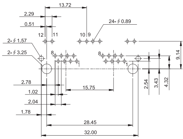
P.C.B LAYOUT/TOP VIEWS
