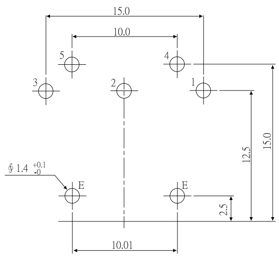
PCB LAYOYT (TOP VIEW)
